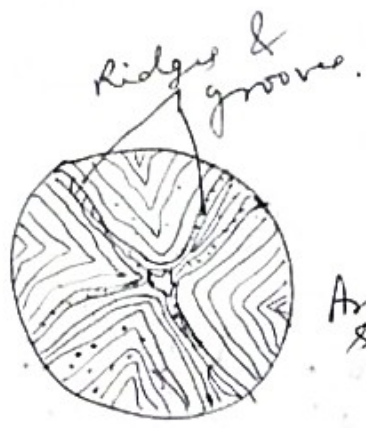
Madreporite in Astria (outerview).
