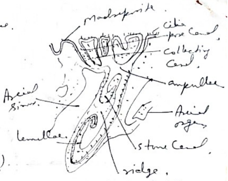
Madreporite in Astria (Vertical Section)
